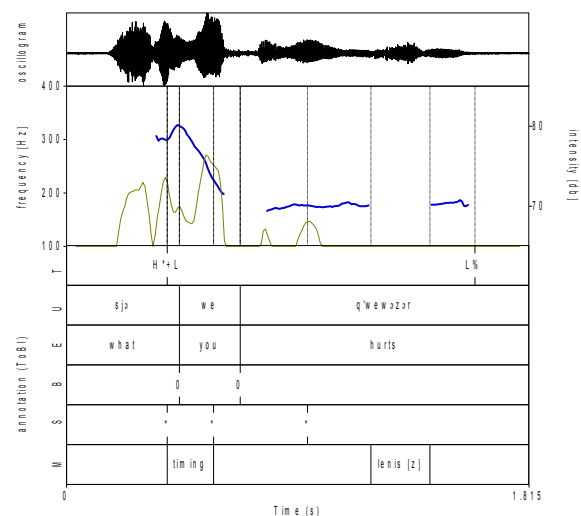
Figure 2: Wh-question intonation.
