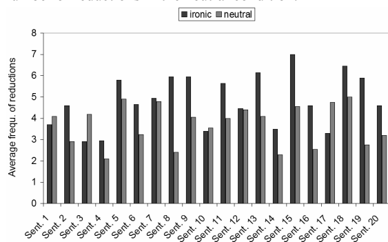
Figure 4: Mean frequency of reductions found across the 10 speakers in the ironic (dark gray) and neutral (light gray) productions of the 20 target sentences.
