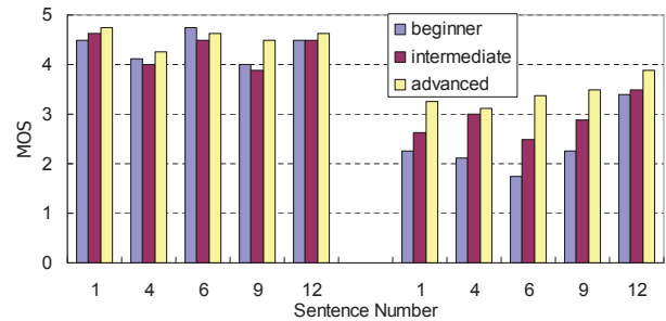
Figure 1: MOS scores on clearness of communication intentions (left) and level of foreign accent (right) of Chinese learners
