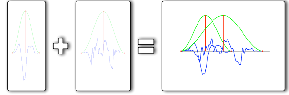
Figure 2: Overlap-add procedure where the successive short-term signals have different widths. Windows are indicated in green and the resulting short-term analysis signal in blue, whereas the GCIs are indicated by a red stem.
