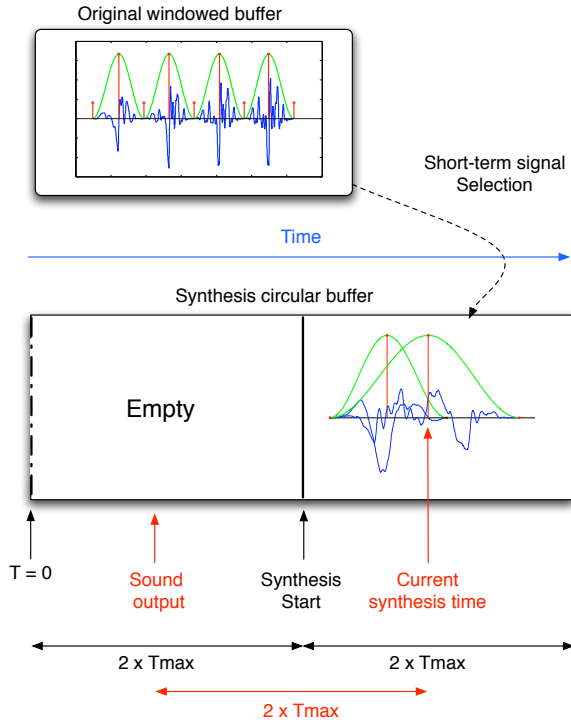
Figure 3: Processing scheme of Calliphony core treatment, from the original windowed speech to the sound card output. On top figure is represented the concatenation of short-term analysis signals, windowed from the original input speech. After selection, these short-term signals are overlapped and added into the circular buffer with a constant delay of 2 \times T_{max} .
