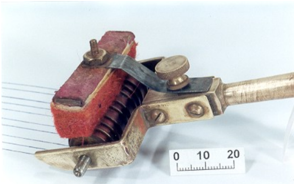
Figure 11: Printing roller for the production of the keyboard-like lines. Photograph of the device in the Dresden collection.
