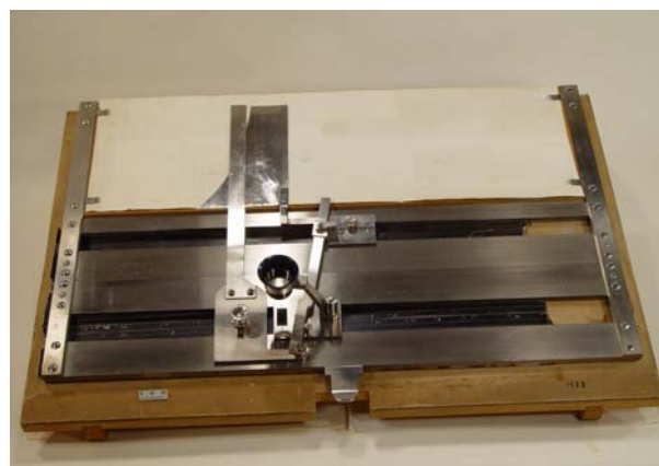
Figure 6: Improved version of the pitch contour measuring apparatus. Original device from the Hamburg Phonetic Institute, now in the Dresden collection.
