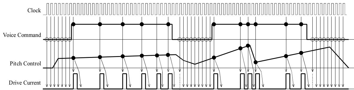
Figure 3: Timing chart of pitch control.
