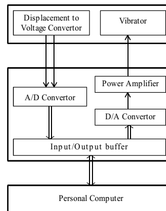
Figure 2: Block diagram of a pilot electrolarynx system.
