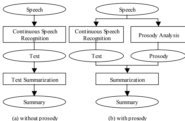
Figure 1: Process of speech summarization.
