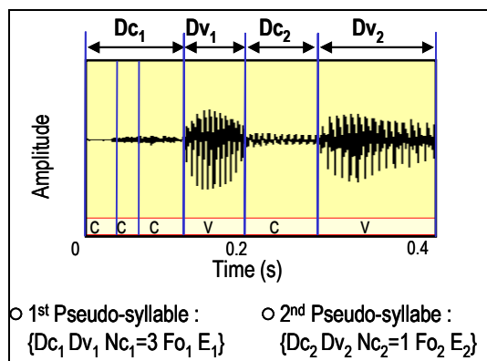
Figure 1: Example of a Vowel/Non-vowel segmentation. The speaker pronounced "... très bo(nne)". Vertical lines are given by the segmentation algorithm.
