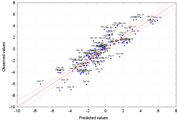
Figure 3: Prediction of the “dynamic level” by 17 acoustic parameters ( R^2=75,39\% ), for the 100 voices.
