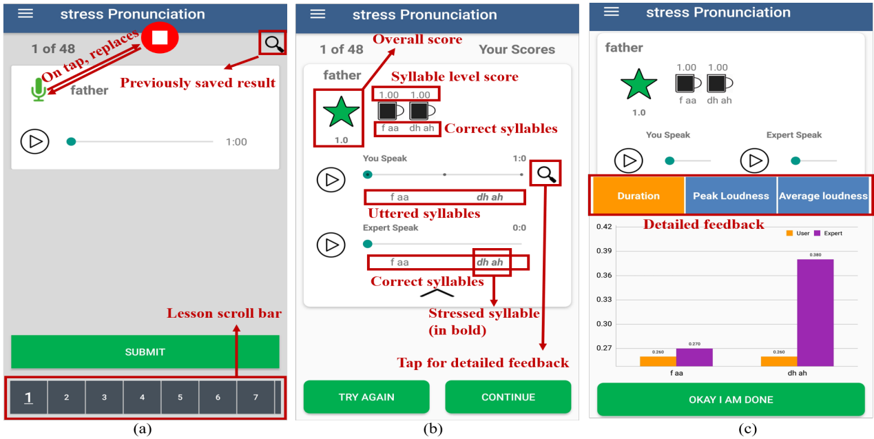
Figure 1: An exemplary user-interface of the stress placement category in voisTUTOR
