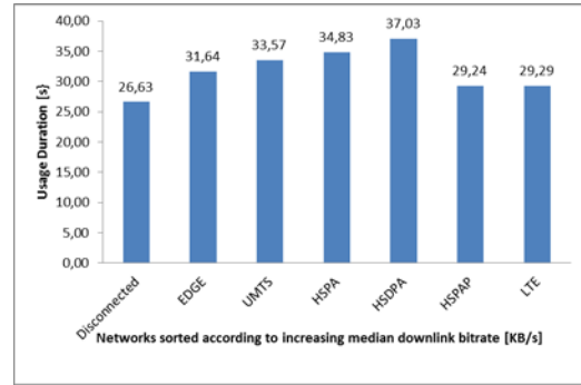
Figure 6: Median session duration of WhatsApp.
