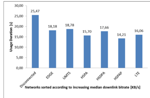
Figure 8: Median session duration of Viber.
