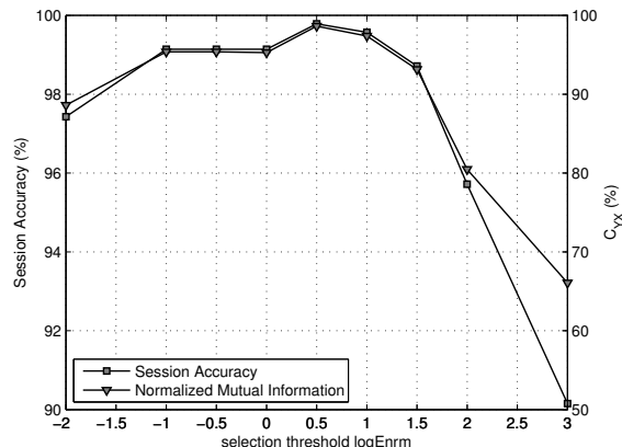
Figure 1: 100\text{-SER} (%) and C_{YX} (%) of the basic GMM ML system on the development data as a function of the frame selection threshold.
