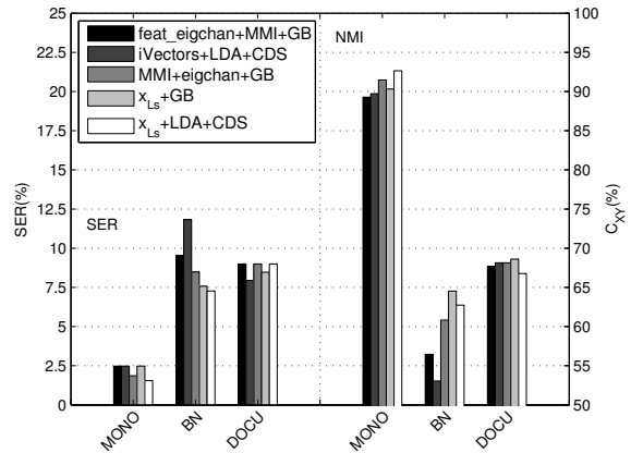
Figure 2: Session Error Rate (%) and Normalized Mutual Information (%) of the two top performing baseline systems vs all the proposed systems on the complete evaluation set.
