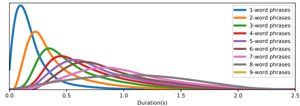
Figure 2: Duration distributions of the phrases in Sub3Vox.
