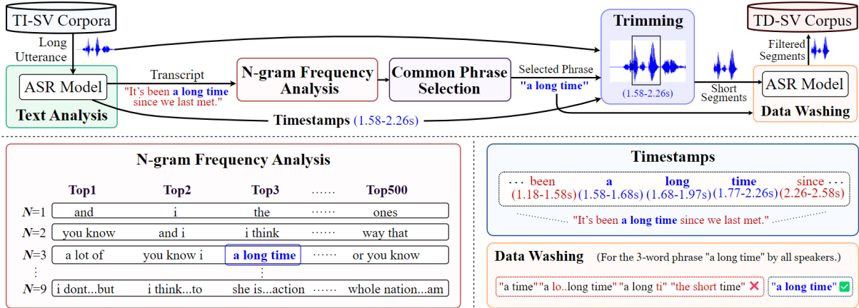
Figure 1: Flowchart of the proposed automatic pipeline for creating a TD-SV corpus from TI-SV corpora.
