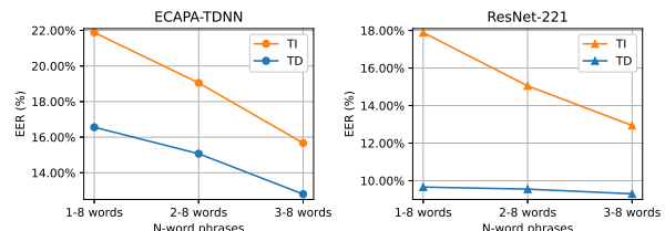
Figure 3: The impact of phrase durations on the performance of TI-SV and TD-SV systems. In the horizontal axis, from left to right, the short phrases (1-word and 2-word phrases) are progressively excluded, leading to longer durations for the test phrases.
