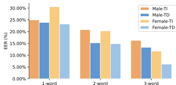
Figure 4: The EER performance of ECAPA1024 LM on Sub3Vox-eval2 for different numbers of words in the test utterances (phrases).
