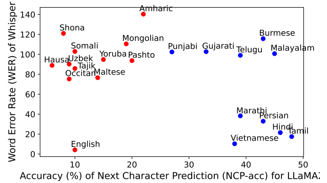
Figure 2: 2D plot comparing the accuracy (%) of LLaMA2 on Next Character Prediction (NCP-acc) with the Word Error Rate (WER %) of Whisper on a subset of languages from FLEURS. The plot serves as a point of reference for selecting languages that might benefit from SALSA. Specifically, we chose languages (colored in blue) that have high NCP-acc and medium to high WER using Whisper.
