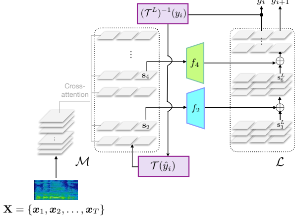
Figure 1: SALSAs overall schematic illustrating the coupling of the ASR model \mathcal{M} and the LLM \mathcal{L} using select projection layers. For the sake of simplicity, we will assume y_i corresponds to a single token in this illustration.
