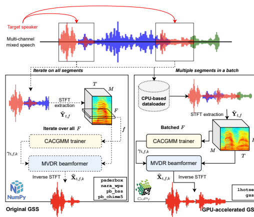
Figure 1: Overview of batch processing for GPU-accelerated GSS. Solid and dotted lines denote GPU-bound and CPU-bound operations, respectively. The WPE module is not shown.
