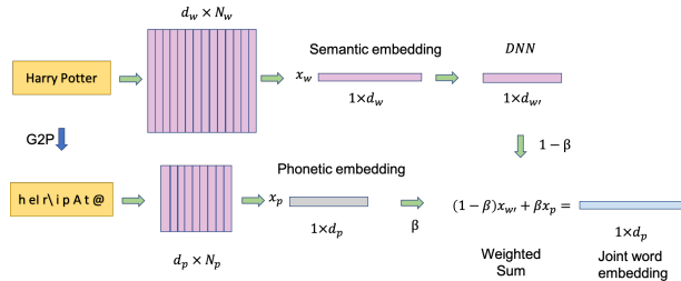
Figure 2: Architecture of Weighted Sum model
