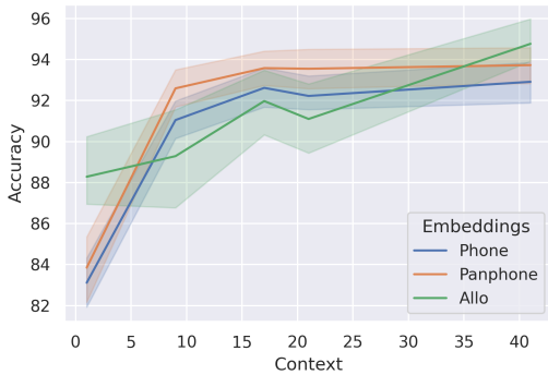
Figure 3: We plot results on Sinhala language when the training size is similar to Tamil. To study the language agnostic embedding claim made by us. We see a similar trend for all the 3 embeddings, which again are derived from Allosaurus tool which is a language independent phone decoder.
