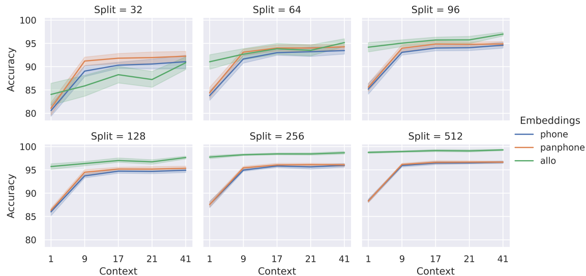
Figure 4: This plot shows the accuracy vs context size on using 3 different embeddings as we increase the number for training examples per intent.
