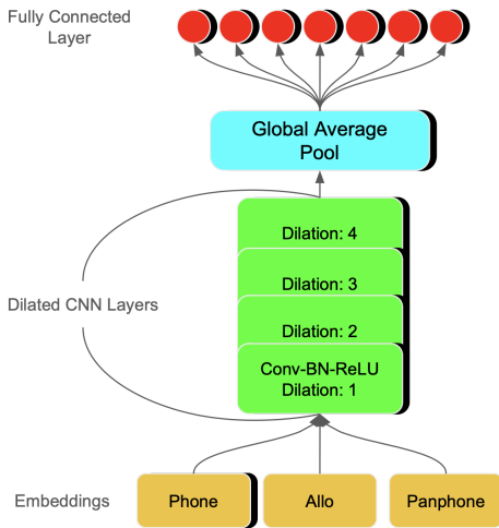
Figure 1: Our proposed choice of method. The reader must keep in mind that the 3 different embeddings are used independently i.e., one at a time, to conduct the 3 different experiments. Any block having a black shadow means the parameters are trainable.
