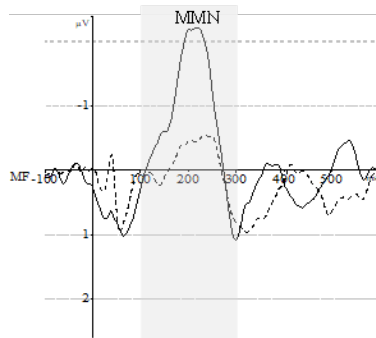
Figure 3: Difference wave showing the response to the pitch deviant for complex waves (solid) and syllables (dashed) at the Middle-Frontal ROI. Figure peak values reflect individual participant variation within the data set. Negative amplitude plotted upwards; figure filtered at 1-25 Hz.
