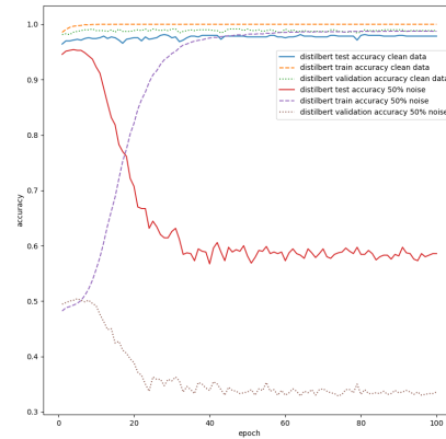
Figure 1: Training, dev, and test accuracy over learning epochs for the SNIPS dataset with 50% label noise
