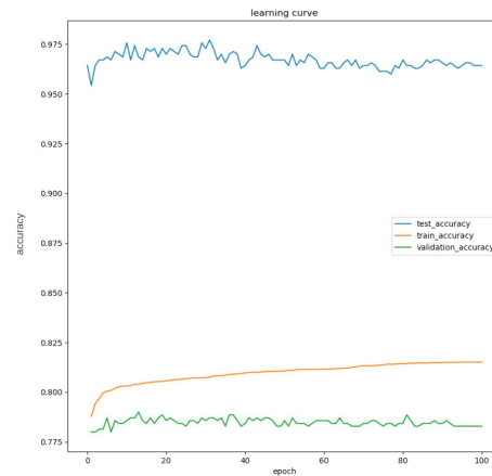
Figure 2: Learning Curve for Robust Loss mitigation method for SNIPS dataset with 20% noise
