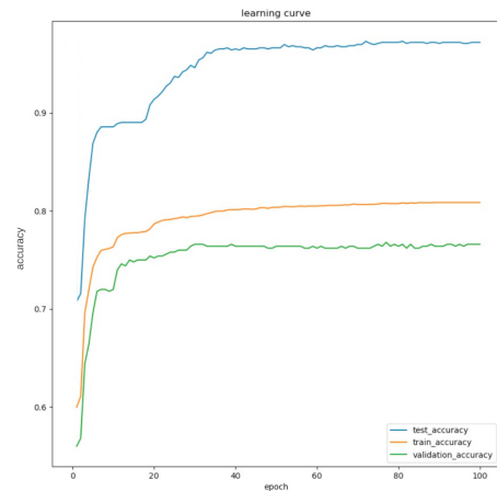
Figure 3: Learning Curve for LIMIT mitigation method for ATIS dataset with 20% noise
