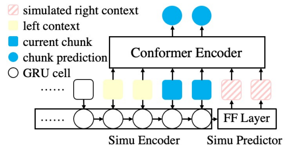
Figure 1: The CUSIDE framework. We split the utterance into non-overlapping chunks, and iteratively run simulation encoder and predictor to simulate a certain number of future frames. Current chunk is spliced with some history frames and the simulated future frames, and they are together fed to the acoustic encoder to produce the prediction for the current chunk. The simulation encoder, predictor, and acoustic encoder are implemented in our experiments as, but generally not limited to, GRU, feed-forward (FF) layer, and Conformer respectively.
