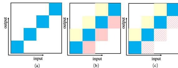
Figure 2: The dependency map of different types of chunking used in inference. (a) Chunking w/o context. (b) Context sensitive chunking with left and right contexts, which are colored with yellow and red, respectively. (c) The proposed chunking with simulated future context. Colored [i, j] denotes whether output[j] depends on input[i] . White means there is no dependency. Dashed means that for output[j] , input[i] is simulated. Here the sizes of left and right context are plotted to be equal to the sizes of the chunk, which is not necessary in practice.
