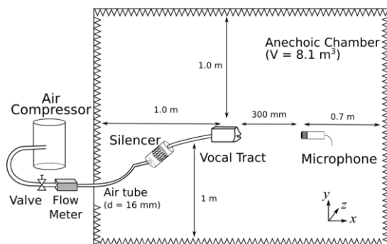
Figure 4: Experimental setups of the sound recording.
