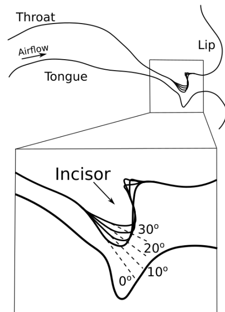
Figure 2: Mid-sagittal plane of the realistic vocal tract and inclined incisor. The original position is at angle 0^\circ and the inclination angle was varied every 10^\circ from 0^\circ to 30^\circ .
