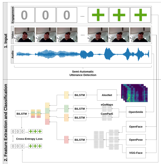
Figure 2: Overview of our proposed system architecture.
