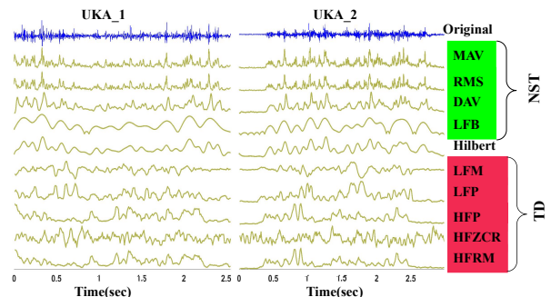
Figure 1: Plots of different features of the EMG signals for 2 subjects (UKA_1 & UKA_2), together with the (time-aligned) original EMG signal
