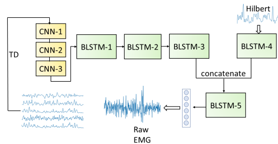
Figure 2: CNN-BLSTM Architecture for Raw EMG reconstruction
