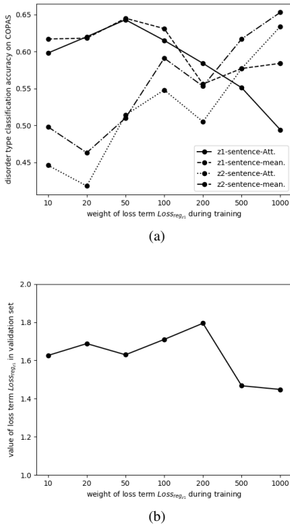
Figure 2: Impact of the weight of loss term Loss_{reg_{z_1}} on (a) disorder type classification accuracy with sentence level z_1 or z_2 input, (b) value of loss term Loss_{reg_{z_1}} in the validation set.
