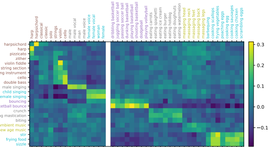
Figure 4: Cosine similarity between some AudioSet sound events (rows) and MagnaTagATune music tags / Kinetics700 actions (columns).
