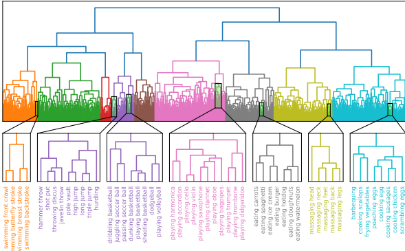
Figure 2: Hierarchical clustering dendrogram of the Kinetics700 actions. To avoid clutter, action names are only shown for some small clusters.
