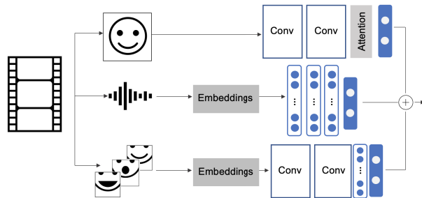
Figure 1: Methodology pipeline.
