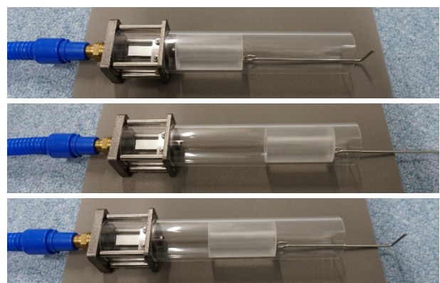
Figure 2: VTM-S20 model (/a/, /i/, and /u/ from the top). The locations of the inner slider inside the outer tube differ for different vowels.
