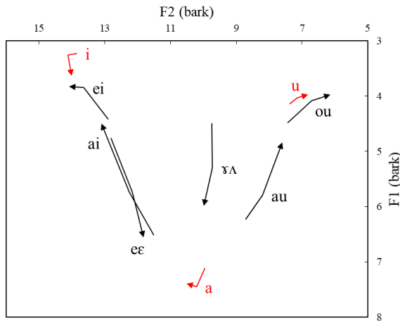
Figure 4 Formant values (bark) of the diphthongs for the male speakers, averaged over speakers and repetitions
