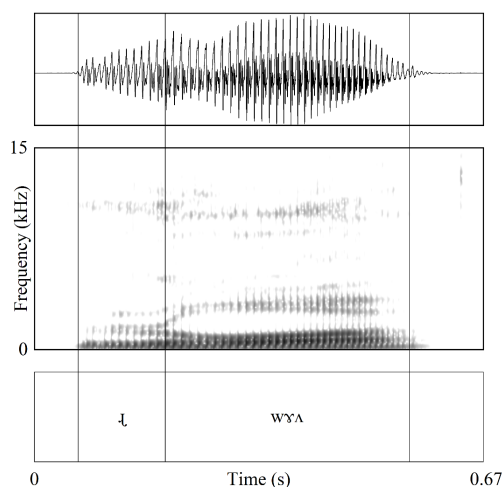
Figure 1 Waveform and spectrogram for the onset /ɿ/ in the word /ɿwʅʌ/ ‘weak’. The upper limit of the spectrogram is set to 15 kHz to allow the examination of the frication noise in the higher frequency range. Pre-emphasis was set at 6.0 db/oct, using the default setting in Praat [12].
