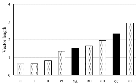
Figure 5 Vector length of the diphthongs
