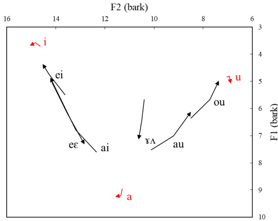
Figure 3 Formant values (bark) of the diphthongs for the female speakers, averaged over speakers and repetitions
