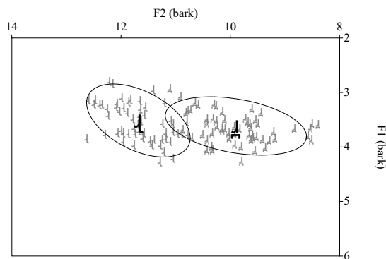
Figure 2 Formant ellipses for approximants [ɹ] and [ɻ]. Data were obtained from ten male speakers. Each speaker has six repetitions per sound. Each repetition is represented as a plot symbol in the F1/F2 plane (bark).
