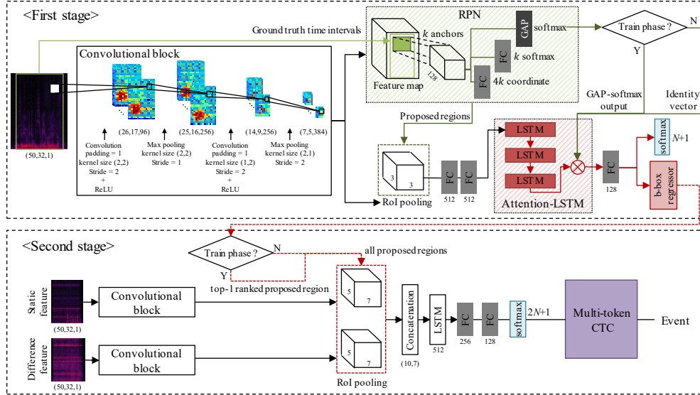
Figure 1: Block diagram of the proposed two-stage polyphonic SED model based on a faster R-CNN and CNN-LSTM with multi-token CTC.
