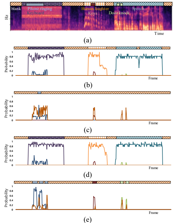
Figure 2: Comparison of decoding paths between the conventional CTC with hinting tolerance of 5 and proposed multi-token CTC for a given audio log-mel spectrogram (a); (b) the first-best path and (c) the second-best path for the conventional CTC; (d) the first-best path and (e) the second-best path for the multi-token CTC.
