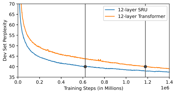
Figure 2: Dev perplexity curves of 12-layer SRU and Transformer models. Vertical lines signify when each model reaches a perplexity of 40. Here perplexity is reported on the combination of dev-clean and dev-other.
