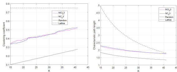
Figure 3. Clustering coefficient and characteristic path length for healthy subjects and patients with MCI as a function for K
