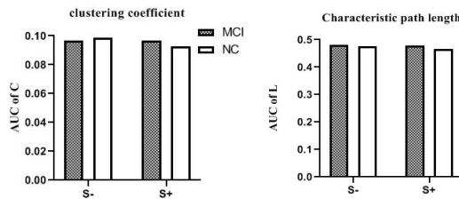
Figure 4. The AUC of clustering coefficient and characteristic path length for healthy subjects and patients with MCI
