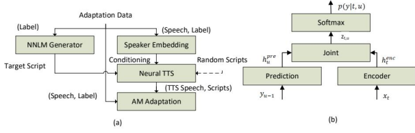
Figure 1: (a) System architecture; (b) RNN-T model structure.
