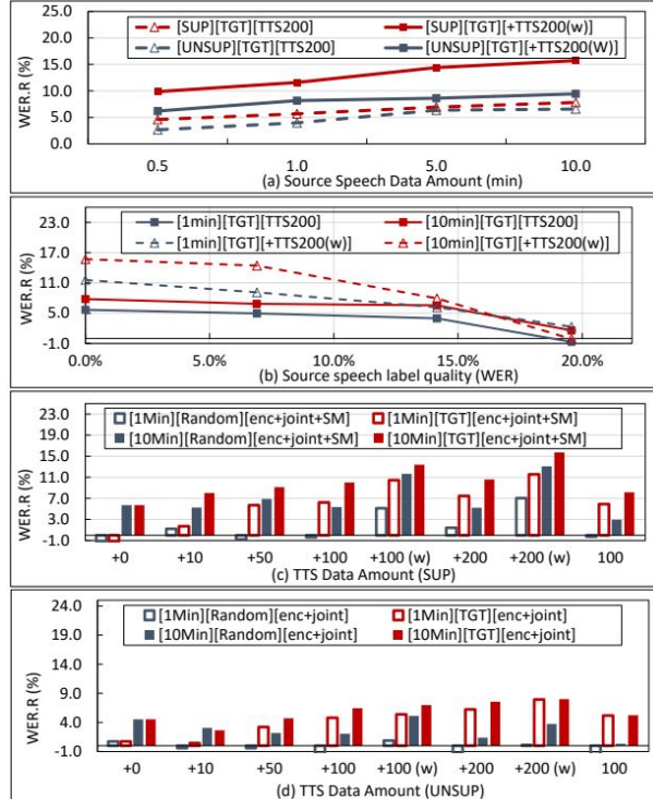
Figure 3: (a) Adaptation performance with respect to source data amount; (b) source label quality; (c-d) TTS data amount.
