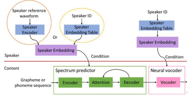
Figure 2: Diagram of personalized speech synthesis.
