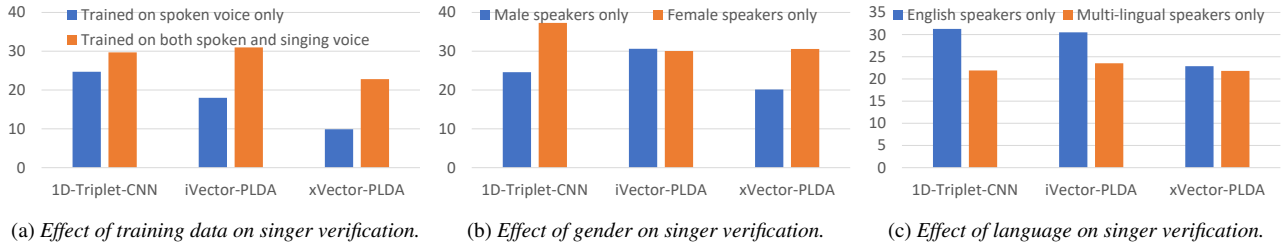
Figure 3: Summary of verification performance (TMR@FMR=1%) across different evaluation conditions on the JukeBox dataset.
