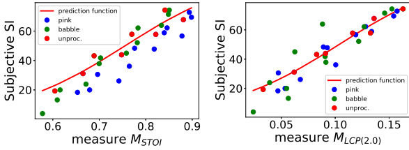
Figure 3: Prediction measures versus subjective SI. Red lines shows the prediction functions
