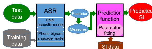
Figure 1: Proposed SI prediction method based on posterior derived from DNN acoustic model
