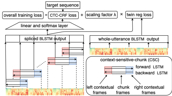
Figure 1: Contextualized Soft Forgetting for streaming ASR.
