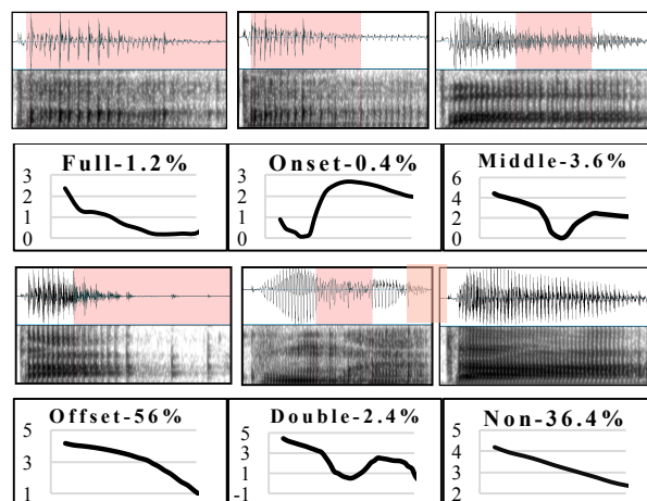
Figure 5: Varieties of glottalized timings and the corresponding pitch contours for T4: [ta4] ('bring') or [ku:v4] ('past') from W1, W5, W1, M1, M2 and W2.
