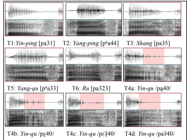
Figure 2: Spectrograms of the Ruokeng tones in carrier sentence: typical cases from a male speaker.
