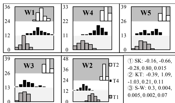
Figure 8: Generational changes of the pitch slope in the modal-voiced portion within T4 (black) by reference to the distribution modes of the falling tone T1 (grey) and the level tone T2 (white).
