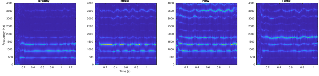
Figure 1: An illustration of SFF spectrograms for breathy, modal, flow and tense phonations for vowel A in Soprano singing category.
