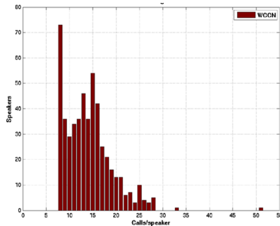
Figure 1: Profile of data available for training the WCCN matrix.
