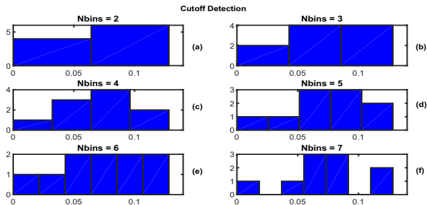
Figure 5: Illustration of the histogram based segregation of candidate peaks corresponding to GCIs and other peaks. Figures (a),(b),(c),(d),(e), and (f) represent the histograms of the peaks for varying bins of 2,3,4,5,6 and 7 respectively.
