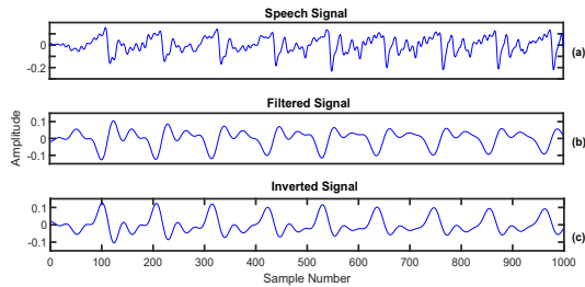
Figure 4: Illustration of inversion process (a) Voiced speech segment, (b) RC filtered signal and (c) inverted RC filtered signal.
