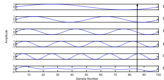
Figure 7: Illustration of the quantitative choice of epoch interval threshold based on sum of sinusoidal harmonics. Figures (a), (b), (c), (d) and (e) represent the sinusoid of 1,2,3,4, and 5 th harmonics of F0 and Figure (f) represents the summation of all the harmonics of F0.
