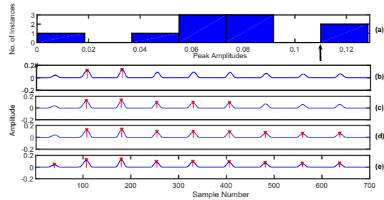
Figure 6: (a) Illustration of candidate GCI locations distributed over a histogram based on peak amplitudes. The black pointer in (a) represents the initial threshold. The candidate GCI locations detected for different thresholds is shown in (b), (c), (d) and (e) respectively.
