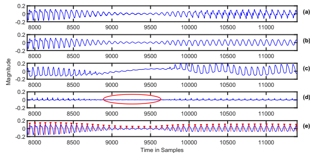
Figure 9: Illustration of a voiced segment representing the vowel transition. Figure (a), (b), (c), (d), and (e) represent the Speech Signal, RCF Signal, EGG Signal, DEGG Signal, and GCIs detected over a RCF signal respectively. The Ellipse in (d) marks the insignificant region in DEGG Signal, even though the excitation is clear from Speech and RCF Signal.
