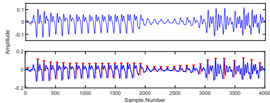
Figure 8: Illustration of the performance of the proposed GCI detection method on weakly voiced region and irregular periodicity regions. Figure (a) represents the speech signal and Figure (b) represents the detected GCIs as vertical markers.
