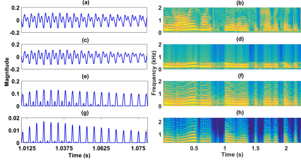
Figure 2: Illustration of RC filtering of speech signal followed by non-linear processing for emphasizing the epoch locations. A segment of speech signal, RC filtered signal, positive clipped and inverted signal, and resulting squared signal is shown in (a), (c), (e) and (g) respectively. The corresponding spectrogram of the time domain signals are shown in (b), (d), (f) and (h) respectively.
