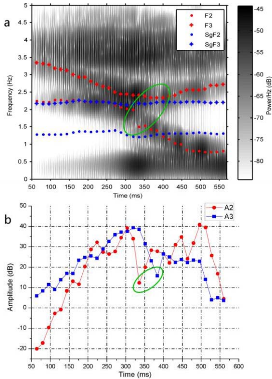
Figure 4: Spectrogram and formant amplitude curves in /iou/ from subject F2. (a) Trajectories of F2, F3, SgF2, SgF3, A2 and A3 on a spectrogram, and (b) A2 and A3 amplitude tracks showing the time lag between F2 and F3 gaps.
