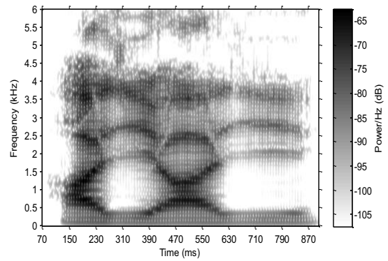
Figure 5: Spectrogram showing the traveling anti-resonance during /aiai/ in a male speaker. Anti-resonance (narrow brighter band) falls from /a/ to /i/ crossing F3 and F2 and rises again in /a/ crossing F2 first.
