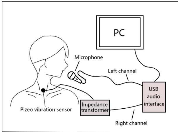
Figure 1: Experimental setup for recording speakers' speech and subglottal resonance. The signal from the piezoelectric vibration sensor was conditioned by a transformer for impedance matching.
