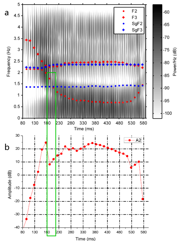
Figure 3: Spectrogram and formant amplitude curve in /iou/ from subject M1 with marking on F2 discontinuity (green rectangle). (a) Trajectories of formants (F2 and F3) and subglottal resonances (SgF2 and SgF3) on a spectrogram, and (b) A2 amplitude curve showing a rapid fall of -16.6 dB at the discontinuity.
