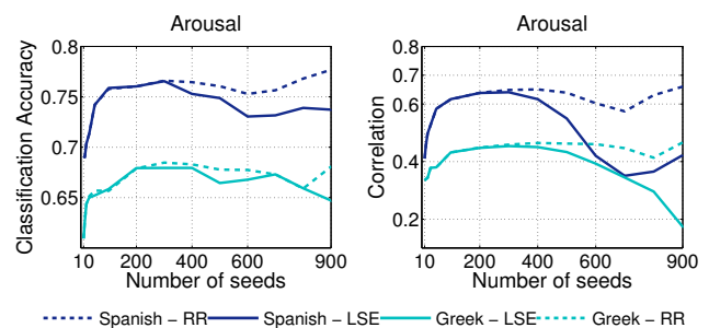
Figure 3: Classification accuracy (left) and correlation (right) for arousal using LSE and RR for the estimation of weights.
