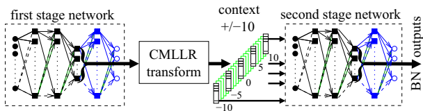
Figure 1: Scheme of Stacked Bottle-Neck Neural Network feature extraction.
