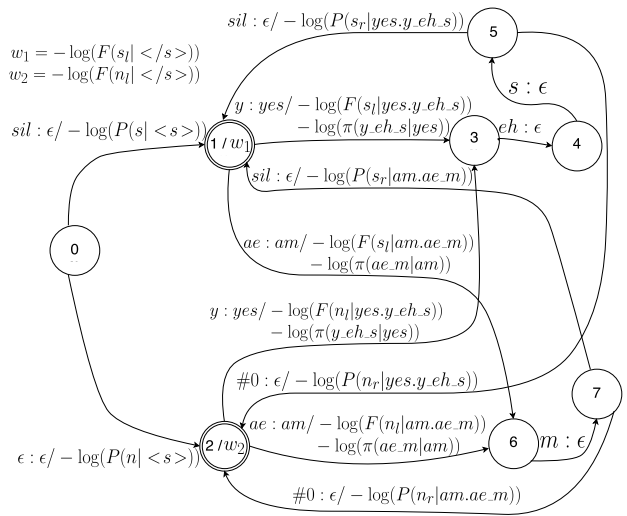
Figure 3: Lexicon FST with word-dependent silence probabilities ( L_3 )
