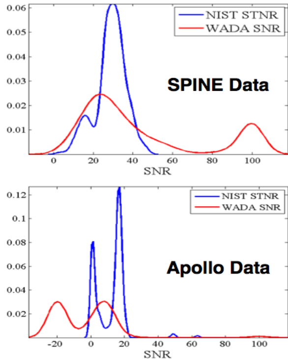
Figure 2: SNR and STNR comparison for SPINE and Apollo data.
