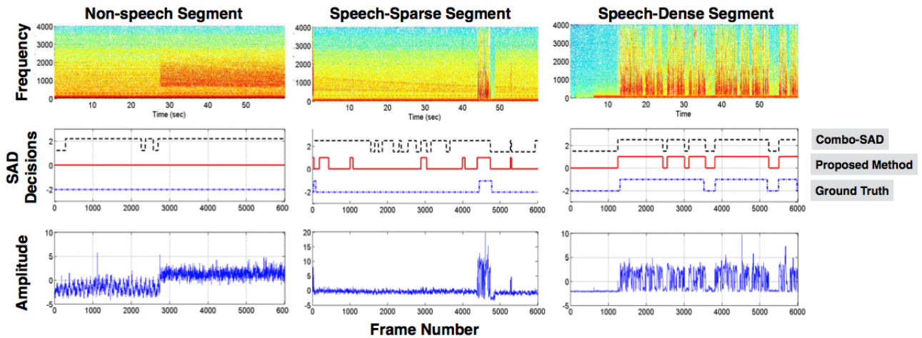
Figure 4: Comparison between proposed method and Combo-SAD on three example files.
