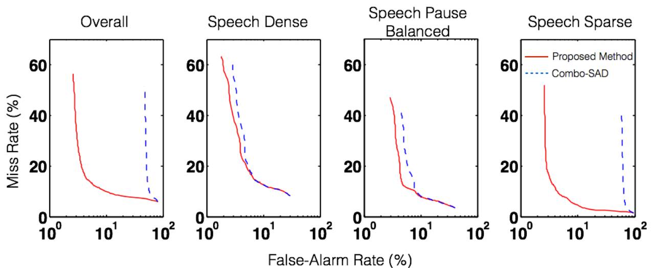
Figure 5: DET curves for APOLLO data utterances.
