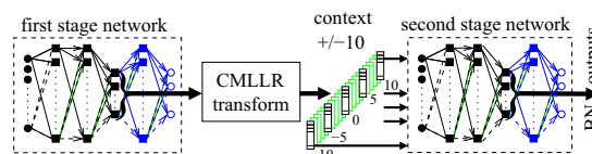
Figure 1: Stacked Bottle-Neck Neural Network feature extraction.
