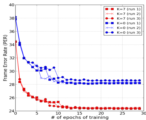
Figure 3: Frame Error Rate (FER) of DART on the TIMIT dev set using DNNs with five hidden layers of 2000 units each. Each model used \pm 7 frames of context. The DNN's were trained to predict \pm 7 frames of context for the multi-frame models ( K = 7 ) and only the central frame for the non-multi-frame models ( K = 0 ).
