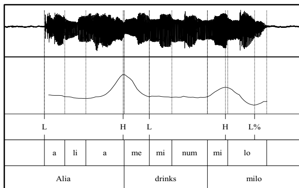
Figure 1: A typical SVO declarative in Malay
