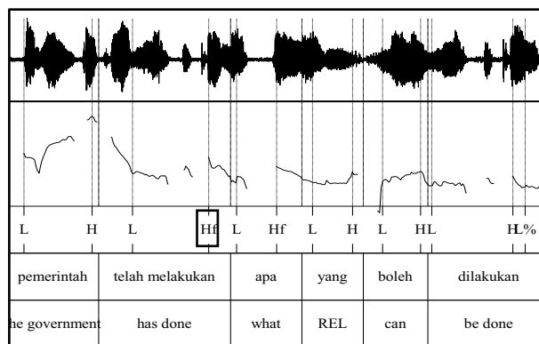
Figure 11: IP containing a verb with suffix -kan
