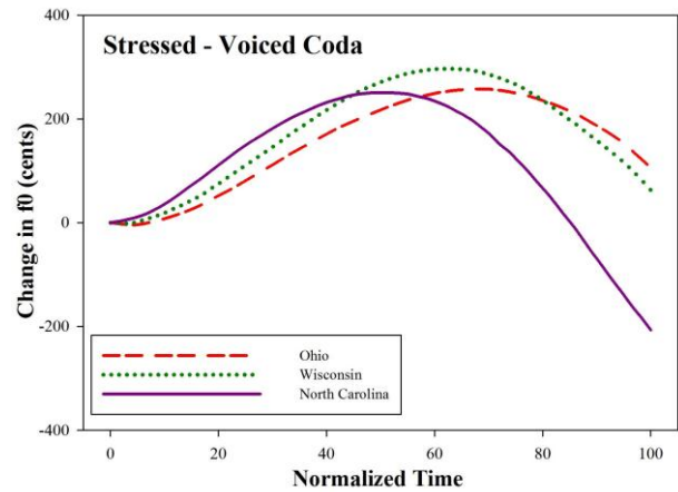
Figure 3: Mean f0 contour for stressed vowels in /b_dz/.
