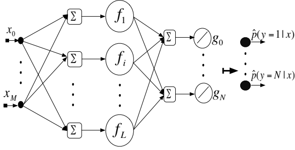
Figure 1: Neural architecture with Hermitian hidden activation functions.
