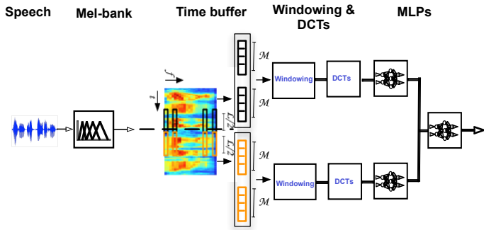
Figure 2: The connectionist architecture used in this work. It is based on the split temporal context idea and three MLPs, as proposed in [5].
