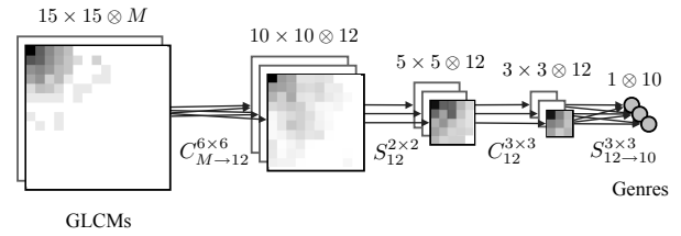
Figure 2: The proposed ConvNets architecture. C_m^{p \times q} and C_m^{p \times q} represent convolutional operations with convolution kernels of size p \times q . S_m^{p \times q} and S_m^{p \times q} are sub-sampling operations with p \times q kernels. The layers corresponding to C_m^{p \times q} or S_m^{p \times q} are fully connected; otherwise connected 1 by 1. i \times j \otimes k above each layer means that the layer has k maps of size i \times j .
