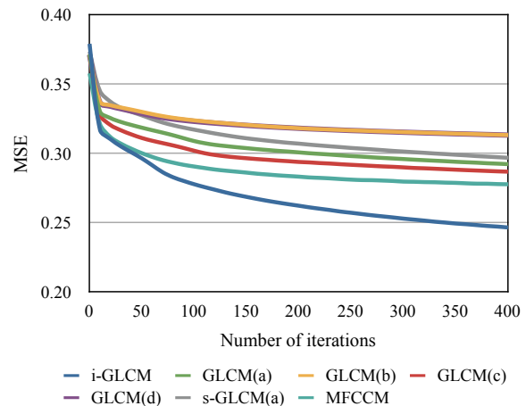
Figure 3: MSE curve over 400 iterations.
